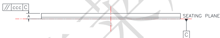
图 5-5 Side View
